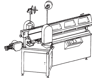
Model II AMPOMATOR CLS Lead-Making Machine 815800-1 (409-5619)
