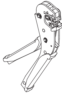
TETRA-CRIMP Hand Crimping Tool 59824-1 (408-2823)
